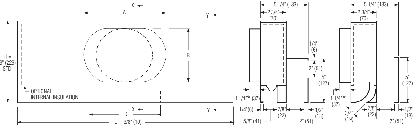
SECTION X-X SR STANDARD SIDE INLET RETURN ILLUSTRATED SECTION Y-Y TR OPTIONAL TOP INLET RETURN ILLUSTRATED
