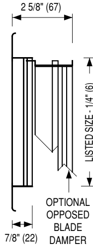
MODEL 6155V Vertical Blades
