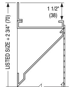
OPTIONAL FLANGED FRAME (FL)
